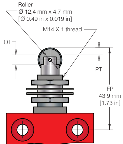
Figure 8. 24CE28 Dimensions
