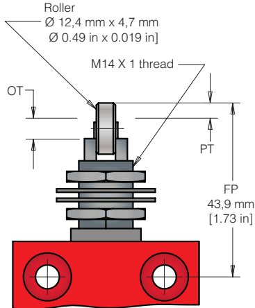
Figure 9. 24CE29 Dimensions
