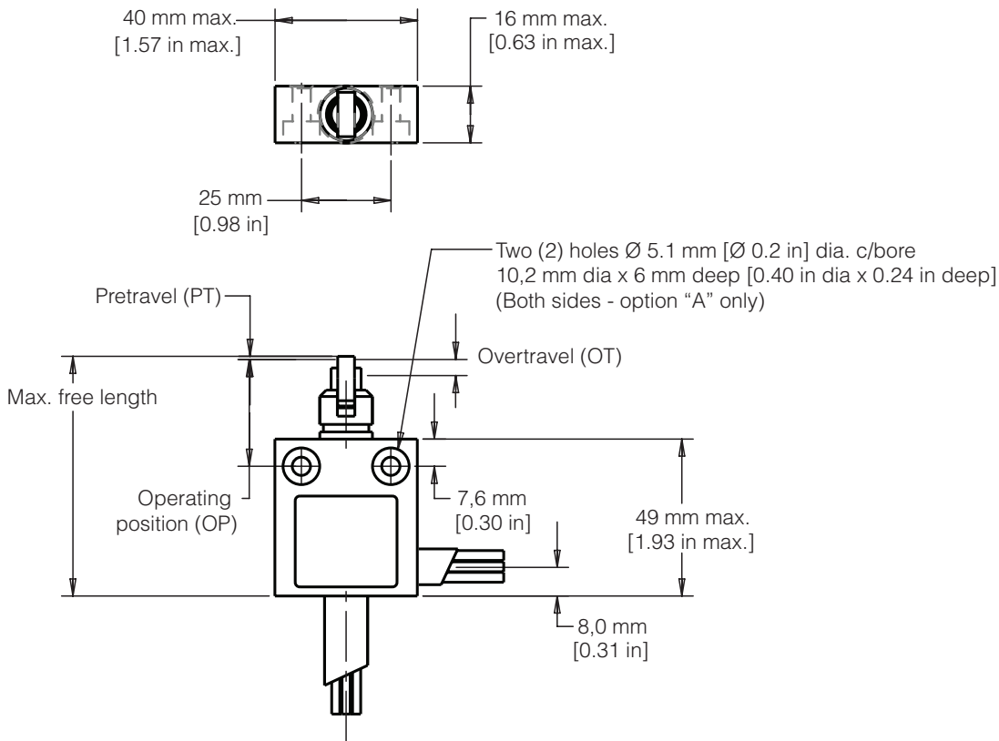
Figure 2. 24CE General Dimensions
