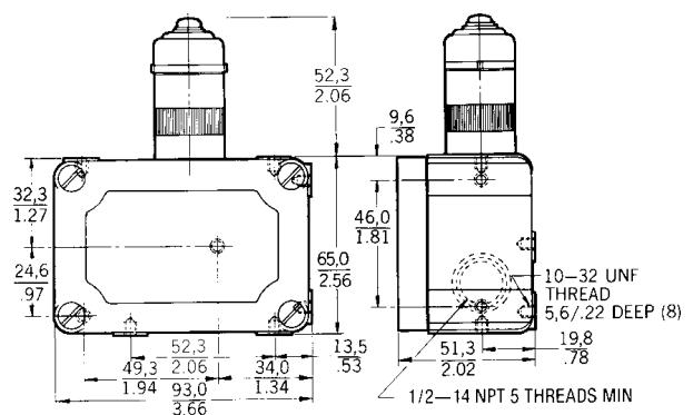
Figure 7. MICRO SWITCH™ EX Series, boot sealed
