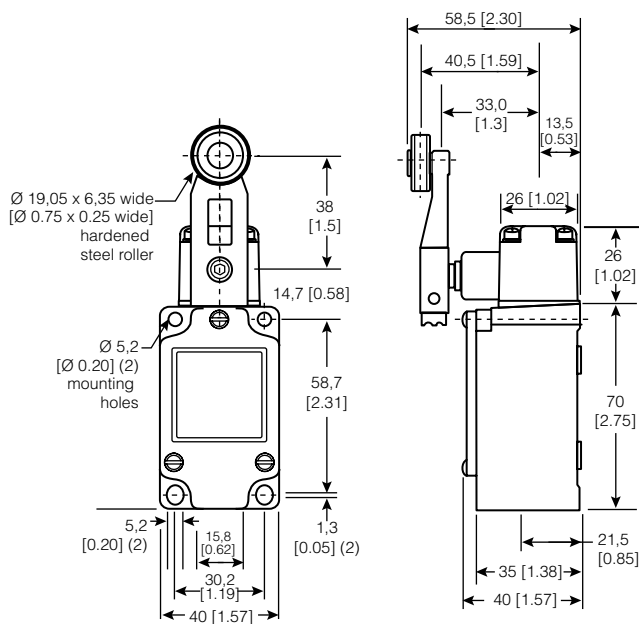
Figure 25. 1LS3-4 Dimensions
