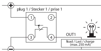
High side switching push/pull outputs
