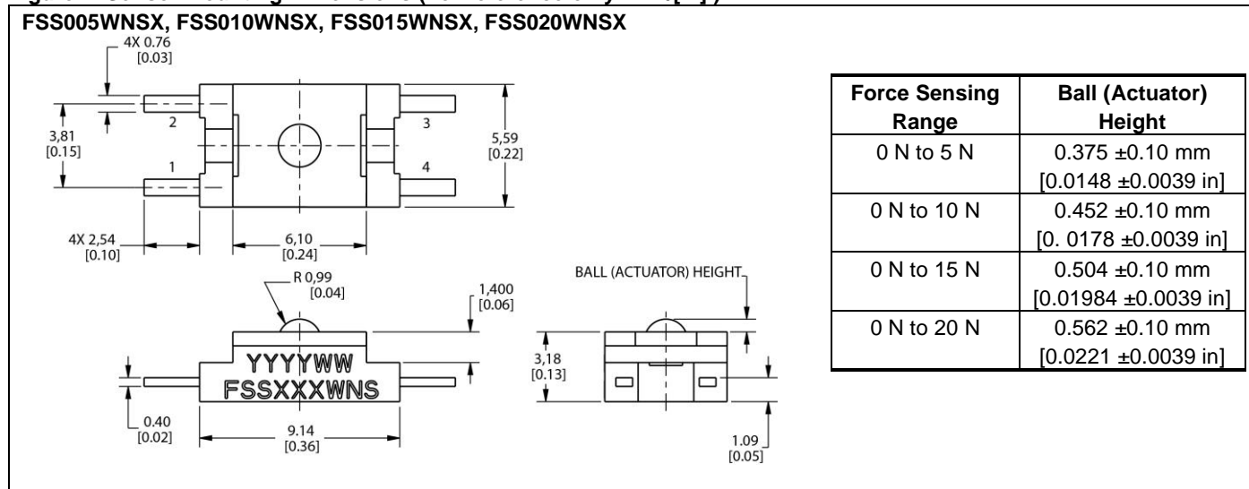
Figure 3. Packaging Dimensions (For reference only.)
