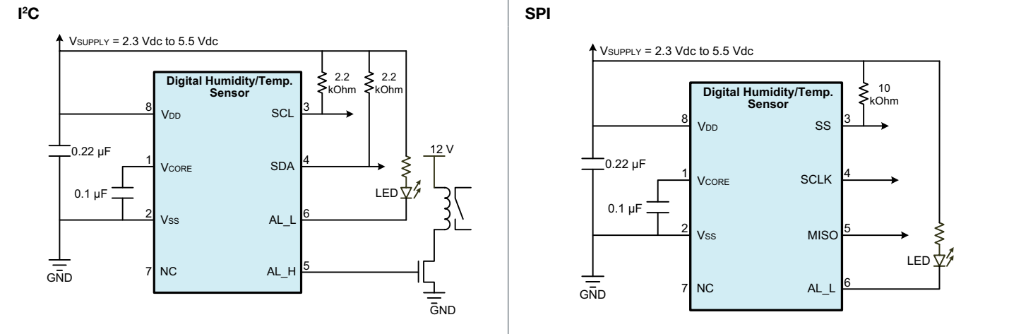
Figure 3. SOIC-8 SMD Typical Application Circuits
