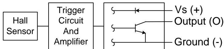
FIGURE 3. CURRENT SINKING OUTPUT DIAGRAM
