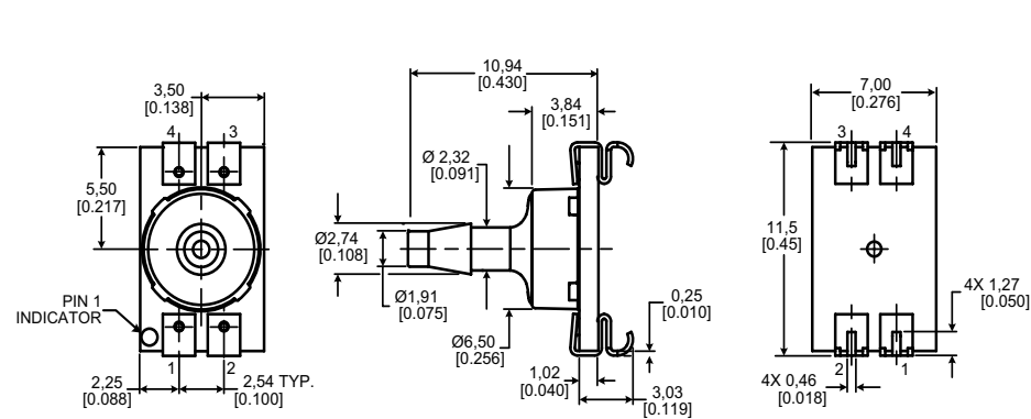
Figure 4. SMT Package Dimensional Drawings (For reference only: mm [in])
