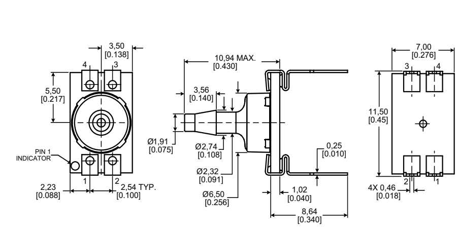
Figure 2. DIP Package Dimensional Drawings (For reference only: mm [in].)
