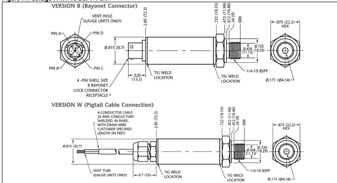
Figure 7. Package 7: 1/4-19 BSPP Port
