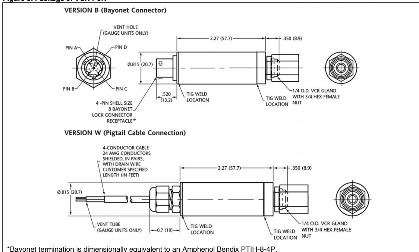
Figure 8. Package 9: VCR Port
